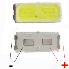
LG 6v 6030 - 6,0x3,0mm LED6024
